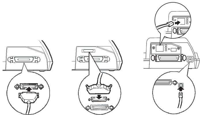
Centronics parallel
